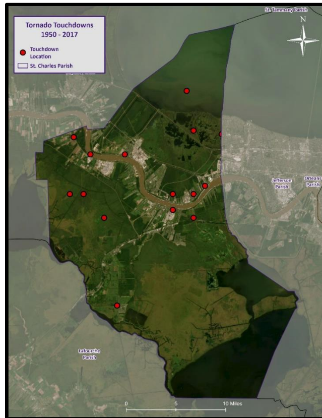
Figure 2-29: Location of Tornadoes to Touchdown in St. Charles Parish (Source: NOAA/SPC Severe Weather Database)
