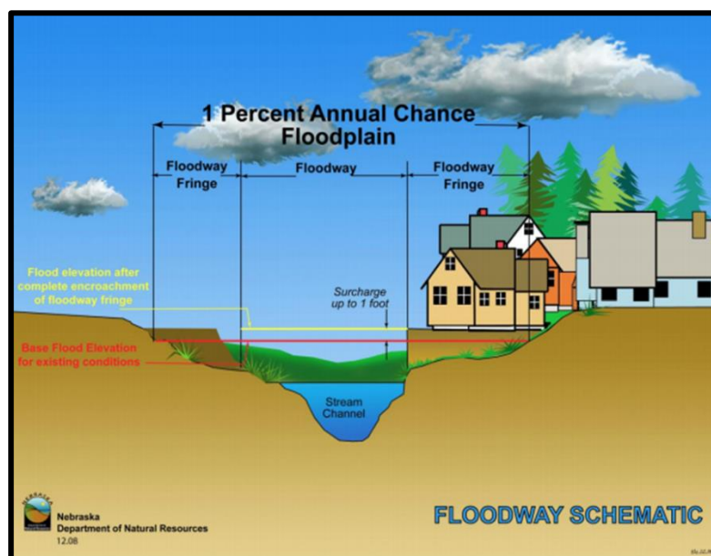
Figure 2-15: Schematic of 100-Year Floodplain. The Special Flood Hazard Area (SFHA) extends to the end of the floodway fringe. (Source: Nebraska Department of Natural Resources)
